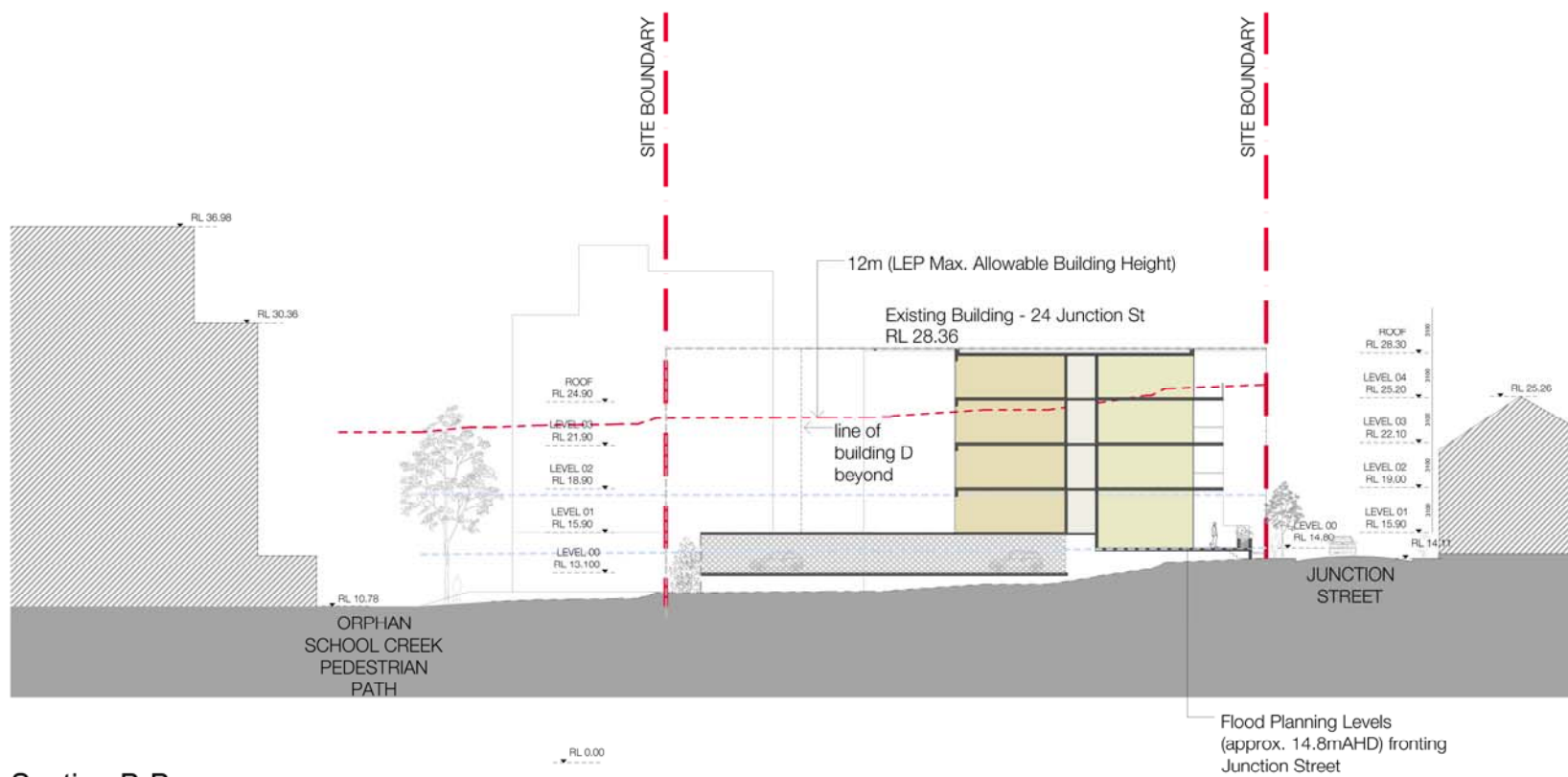
Section B-B
